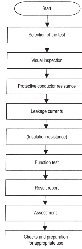
Test sequence according to DIN VDE 0751-1/EN 62353
