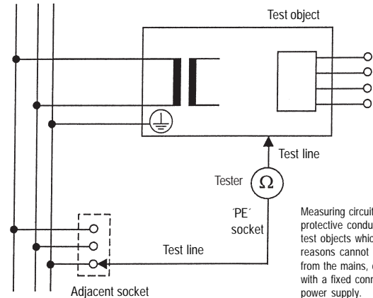
Protective conductor resistance PC I, Diagram C2
