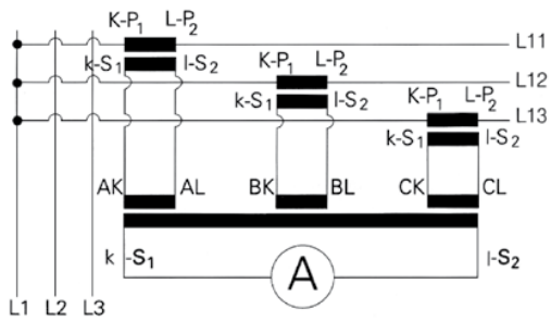
Connection diagram
